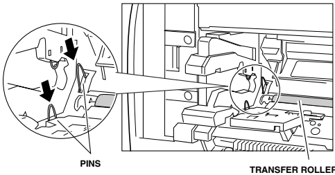
TRANSFER ROLLER
